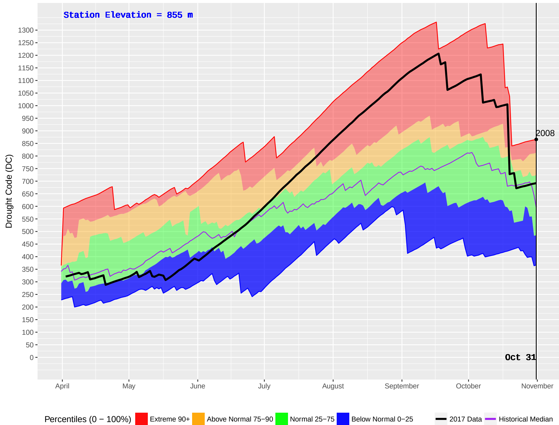
AUGUST LAKE (836) : Historical (2003–2016) and Current (2017) Noon Drought Code (DC)
