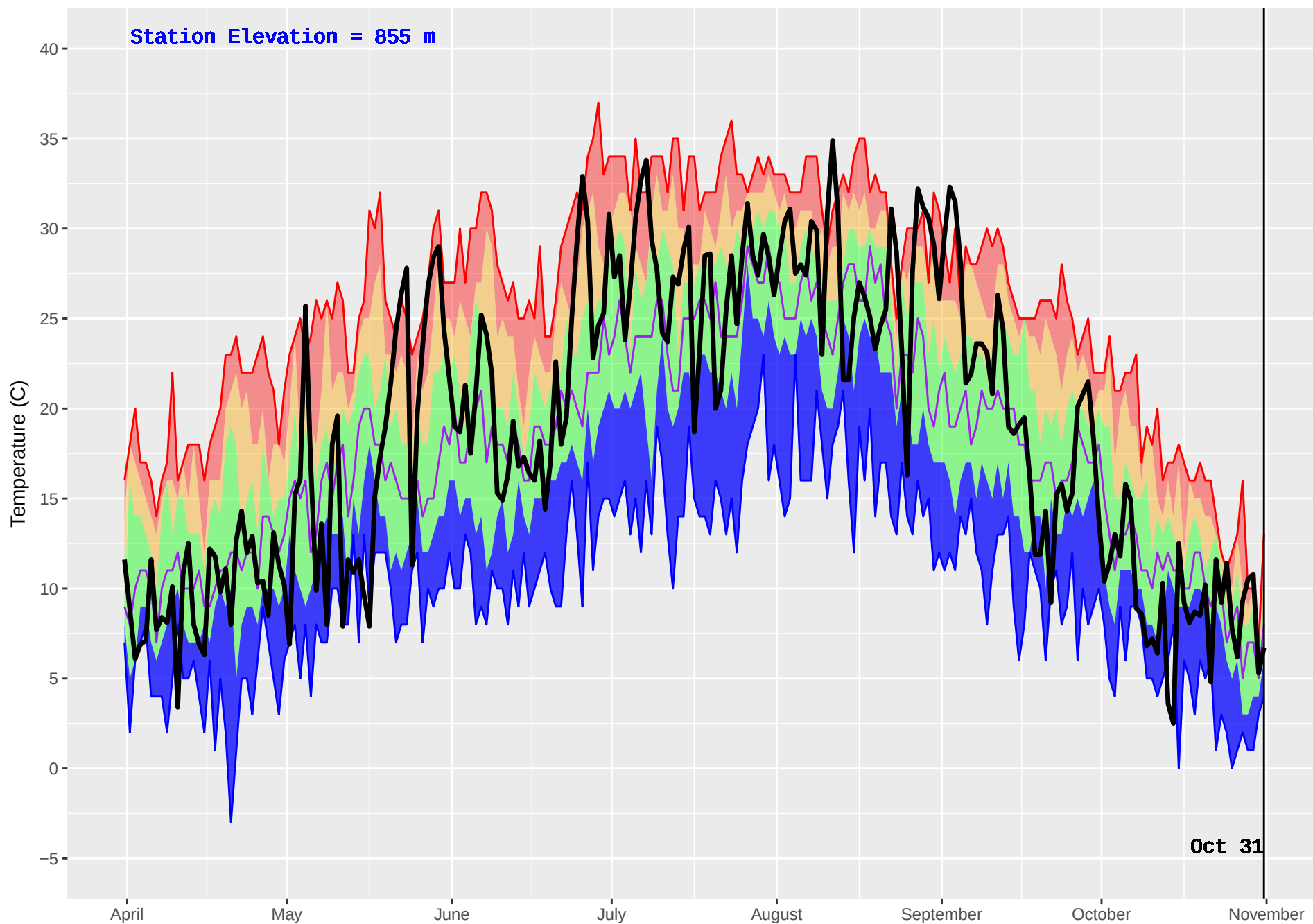
AUGUST LAKE (836) : Historical (2003–2016) and Current (2017) Noon Temperature
